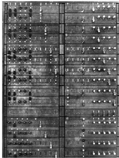
◀ Colossus K2 switch panel showing switches for specifying the algorithm (left) and the counters to be selected (right)
